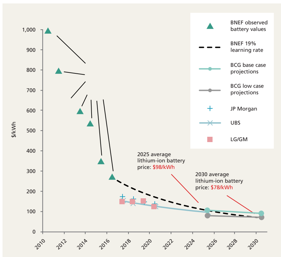
Figure 3: Battery cell cost projections, 2010-2030 2,3
